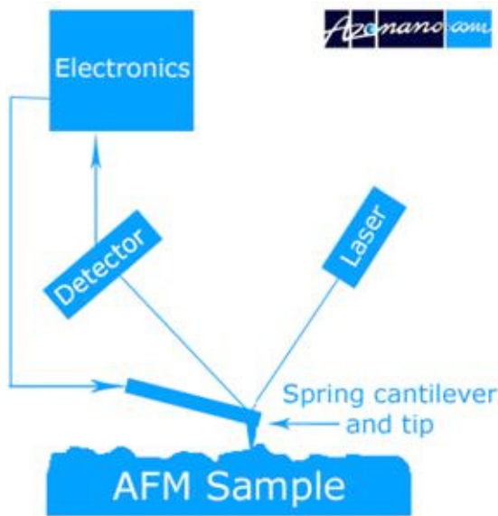
Figure 4: The AFM Principle.
