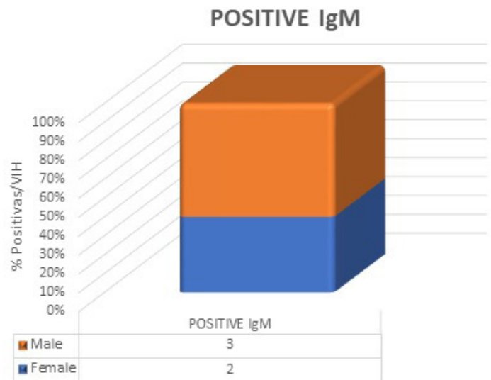
Figure 2: Positive IgM.
