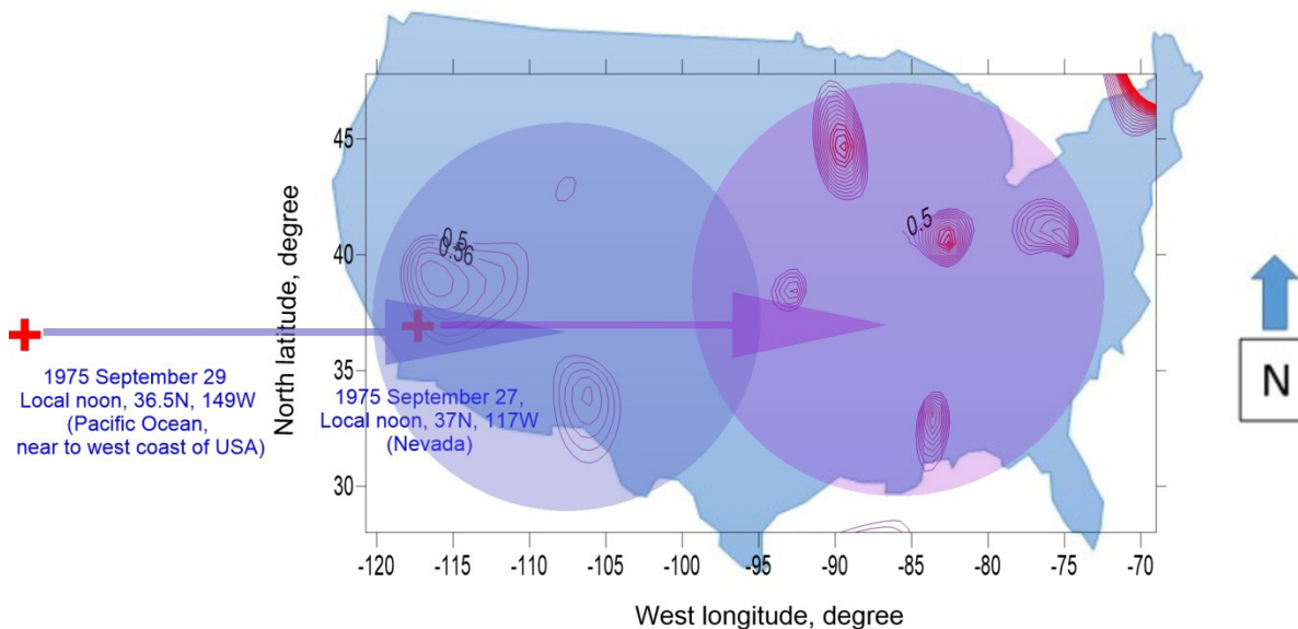
Figure 20: Example of the influence of two pulses of alpha particles. One was recorded on 27 September 1975 with a point of registration 37°N, 117°W over the western US. Its corresponding death spot is located 30° east, covering the eastern United States. The other pulse had a registration point in the Pacific Ocean on September 29, 1975. Its corresponding death spot was located 30° east, covering the western United States.
