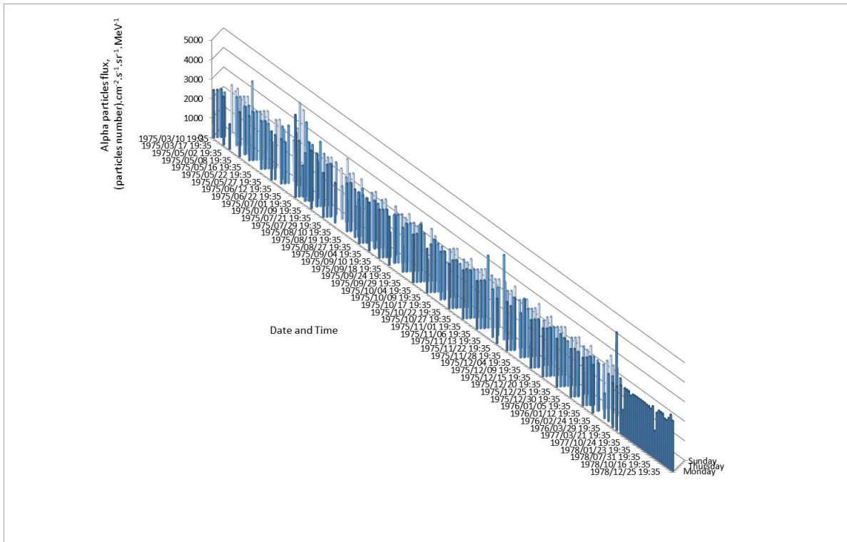
Figure 13: For the survey period of years 1974 – 1979, pulses of alpha radiation with a registration time of 19:35 UTC have an invariable magnitude for large time intervals and change their periodicity from daily to weekly, within the operation of the same satellite, SMS-02.
