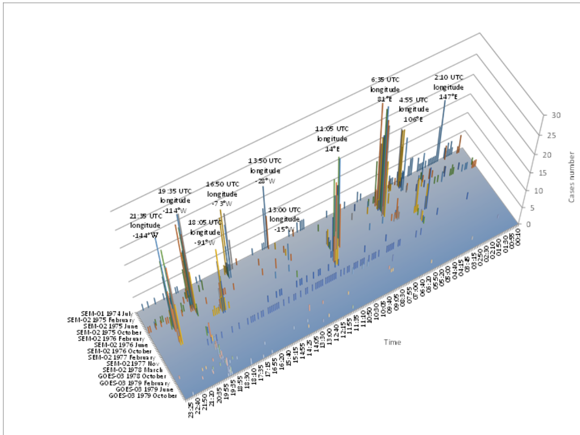
Figure 16: Series of pulses of alpha radiation recorded by a satellite in Earth orbit with the longitude of their point of registration. The most numerous are the series with a registration point over China, the European Atlantic coast, the Western regions of the USA, and the eastern Pacific.
