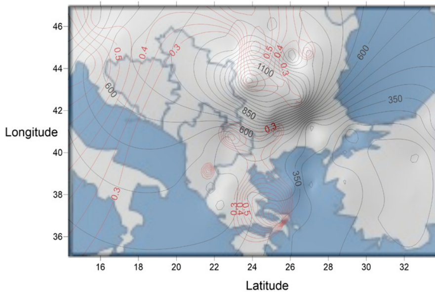
Figure 2: Balkans, a mortality rate (black isolines) from diseases of the circulatory system (I00-I99) and its correlation with annual alpha particle flux (red isolines).
