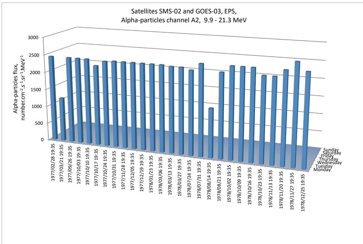
Figure 14: Pulses of alpha radiation recorded by a satellite at 19:35 UTC after February 1977 are strictly periodic with a period of one week, for long intervals they do not change in magnitude and do kill people on the Earth's surface.
