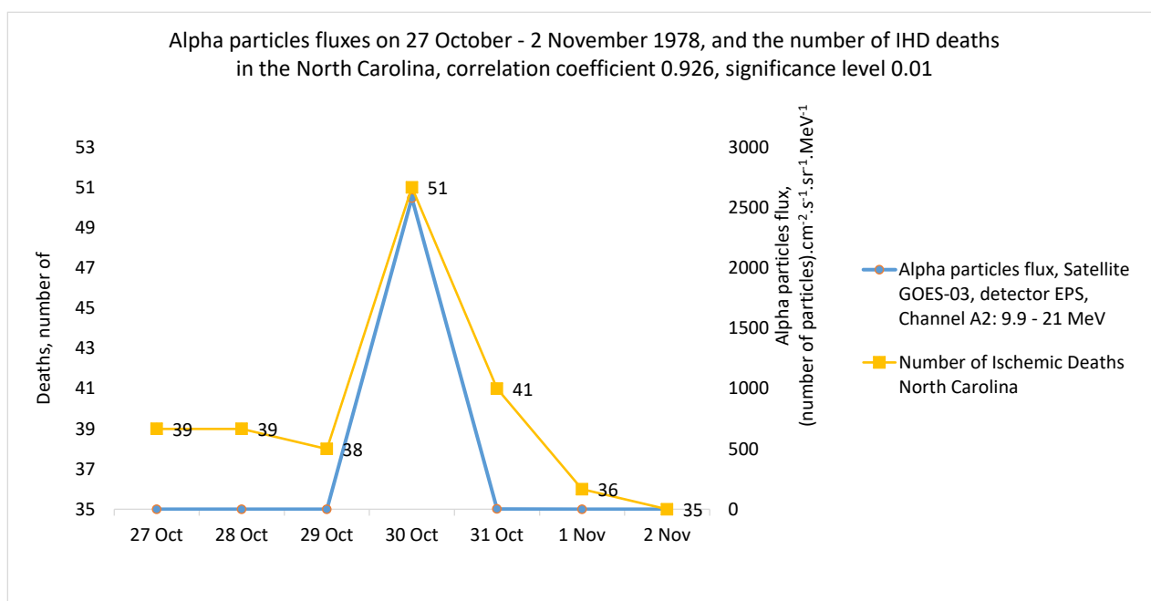
Figure 11: Between the fluxes of alpha particles with energies between 9.9 and 21.3 MeV for the seven-day interval October 27 th – November 2 nd , 1978 recorded by channel A2 of the EPS sensor on board the GOES-03 satellite and the number of IHD deaths in North Carolina for the same interval has a high, statistically significant correlation.
