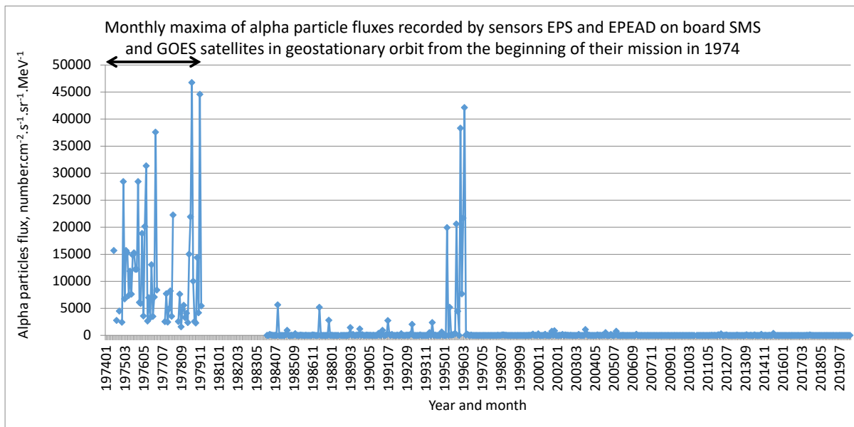
Figure 5: Monthly maxima in the recorded alpha particle fluxes during the interval 1974 – 2019. There are no data for the interval of years 1980 – 1983.
