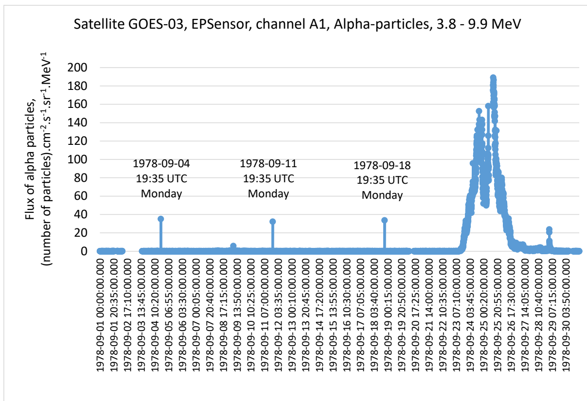
Figure 7: Fluxes of alpha particles with energies between 3.8 and 9.9 MeV were recorded in September 1978 by channel A1 of the EPS sensor on board the GOES-03 satellite.
