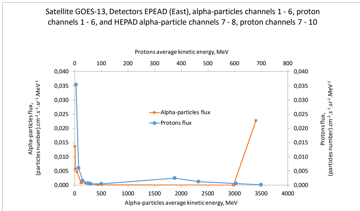
Figure 8: Averaged data for December 2017 from the GOES-13 satellite shows that alpha particles are the only positively charged particles that have energies above a few GeV, allowing them to penetrate the Earth's surface.
