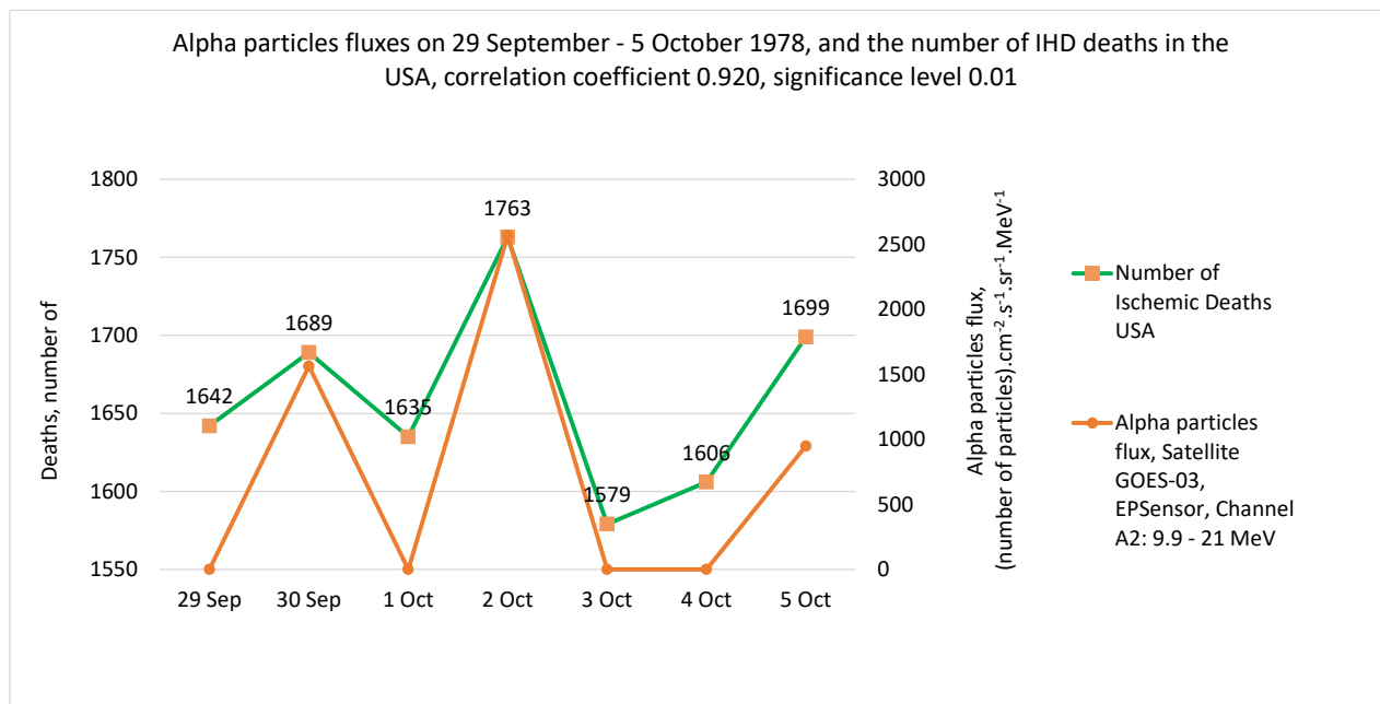
Figure 10: Between the fluxes of alpha particles with energies between 9.9 and 21.3 MeV for the seven-day interval September 29 – October 5, 1978, recorded by channel A2 of the EPS sensor on board the GOES-03 satellite and the number of IHD deaths in the United States for the same interval there is a high, statistically significant correlation.
