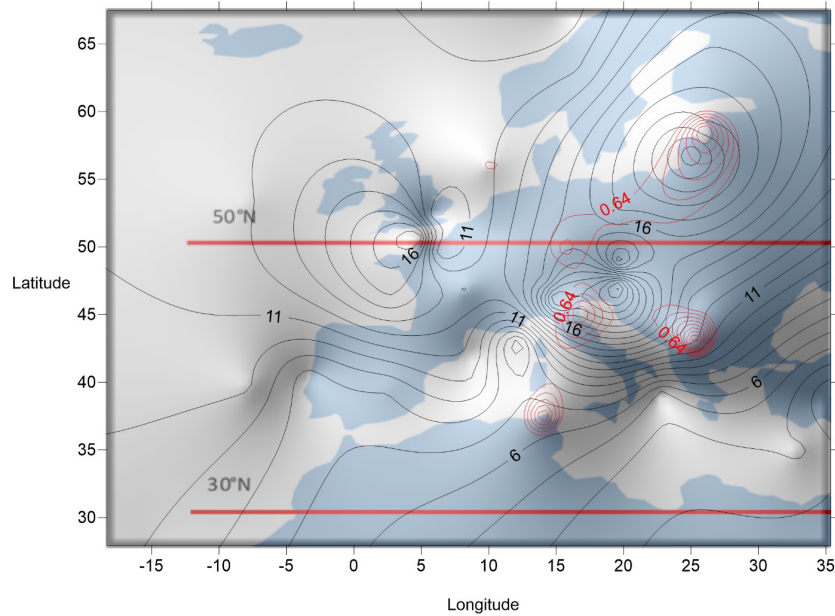
Figure 4: Between mortality from Intentional self-harm (ICD-10, codes X60-X84, Y87) for Europe and the Mediterranean (black isolines) and the annual alpha particles flux reaching Earth's orbit there is a large, statistically significant correlation (red isolines).
