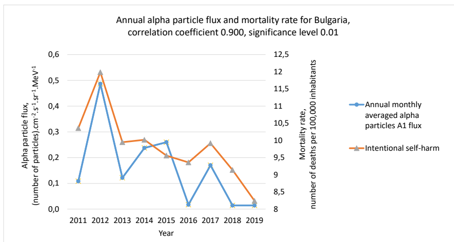
Figure 3: Between the mortality rate from Intentional self-harm (ICD-10, codes X60-X84, Y87) in Bulgaria and the annual alpha particle flux reaching Earth's orbit, there is a large, statistically significant correlation.
