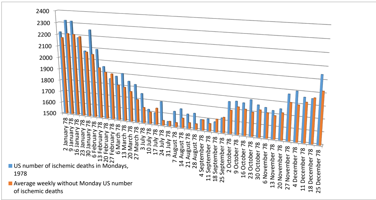
Figure 15: Between the number of deaths in the United States on Mondays in 1978 when pulses of alpha particles were recorded from the series with a time of registration at 19:35 UTC (Figures 13 and 14) and the average number of deaths on the other days of the week there is a statistically significantly different from zero difference.
